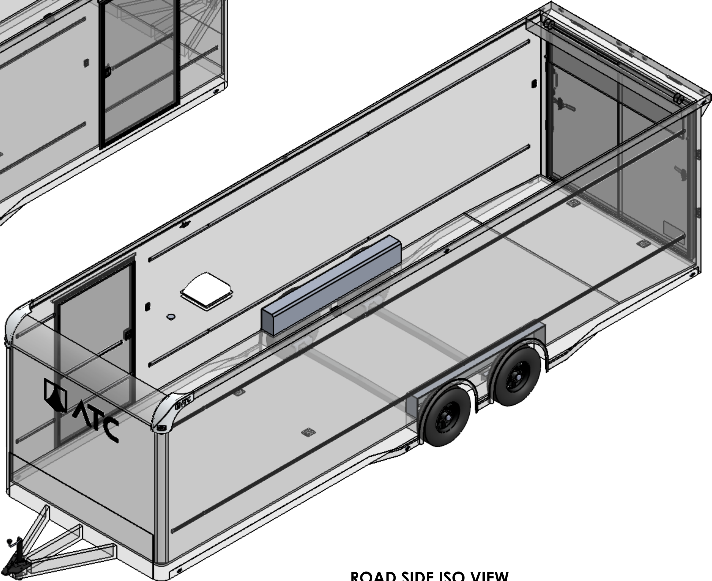
ROAD SIDE ISO VIEW
