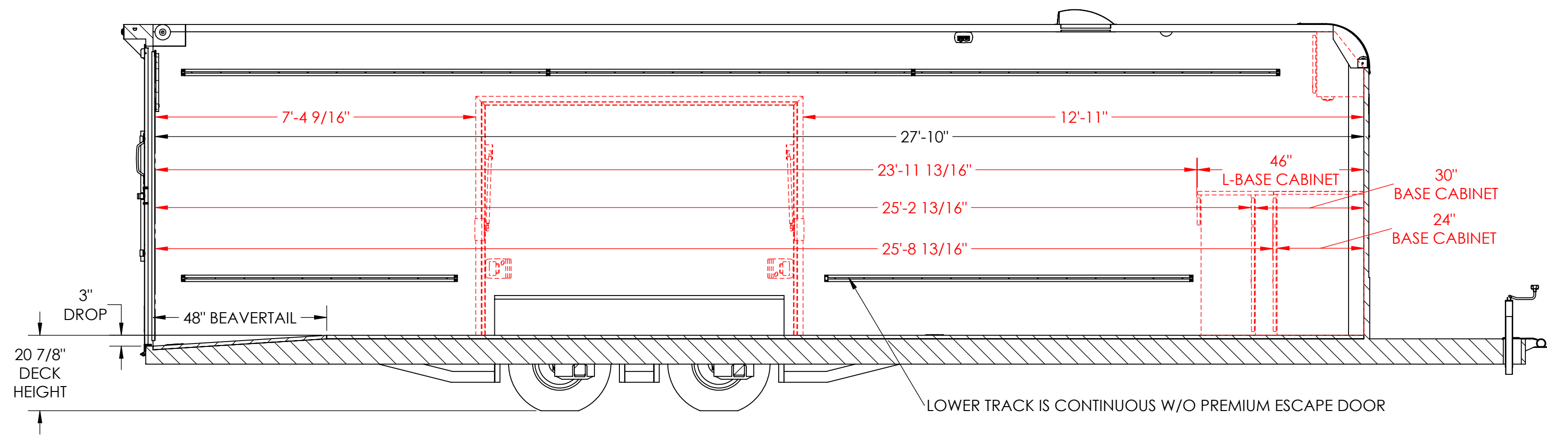
INTERIOR ROAD SIDE SECTION A-A
