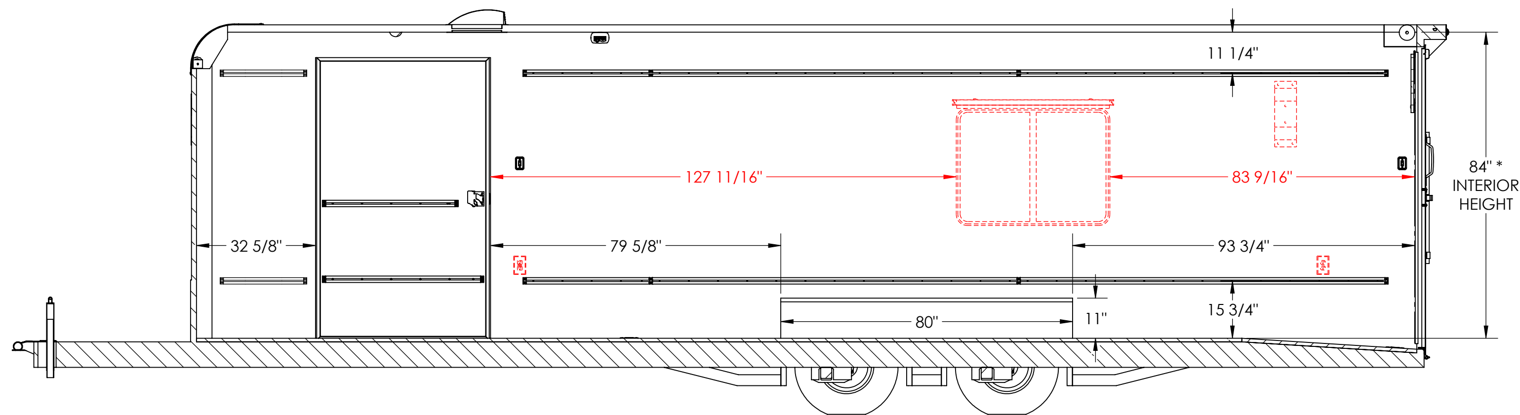
INTERIOR CURB SIDE SECTION B-B
