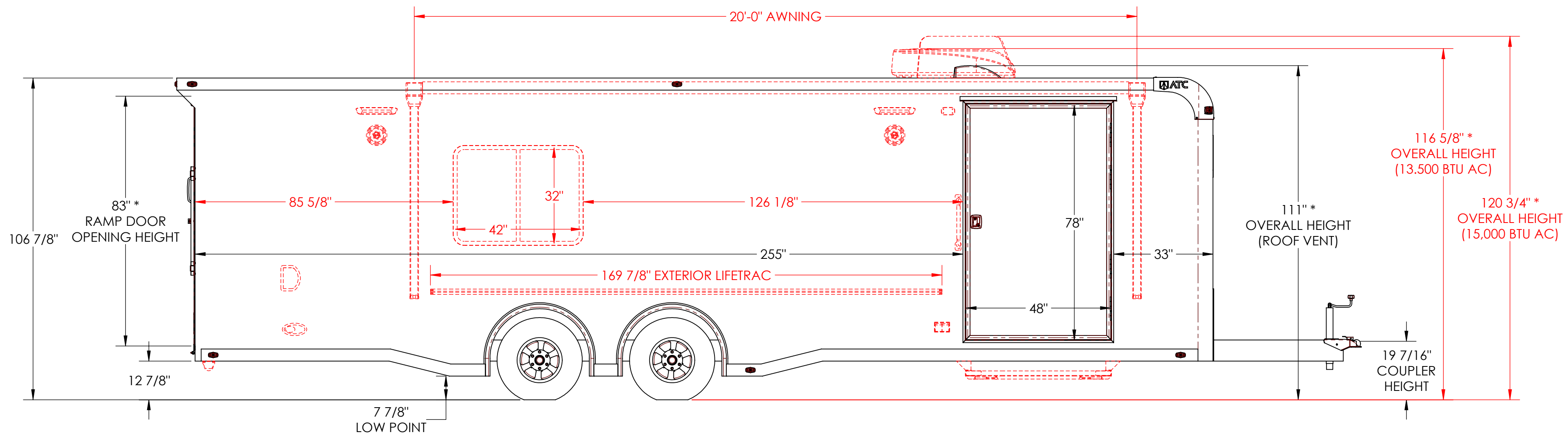
EXTERIOR ROAD SIDE
