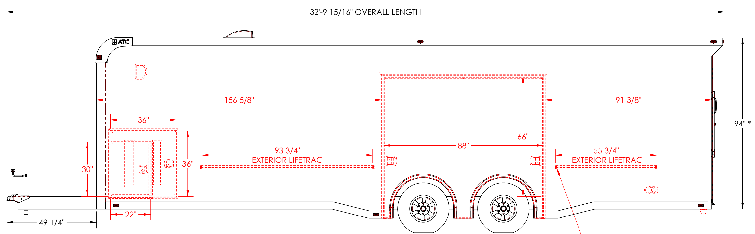
EXTERIOR CURB SIDE
